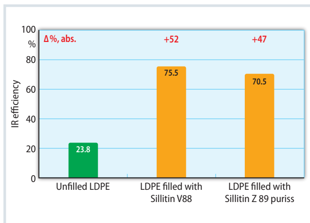
Fig. 4. The IR efficiency of the film rises markedly with addition of Neuburg siliceous earth. To an extent depending on the filler, the increase is 47 to 52 %.
